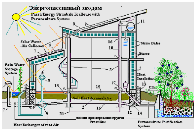
Figure 1. Energy-passive eco-home developed for the project “Eco-houses with “0” energy level, built of natural materials”, Minsk, 1998.
